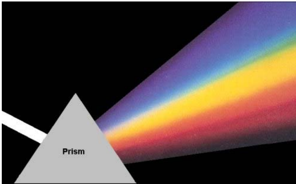
Figure 8. Radio waves are dispersed by the ionosphere just like light through a prism
